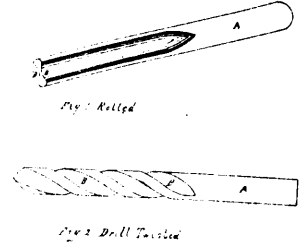
9647 Graham's Art of Manufacturing Twist Drills.
