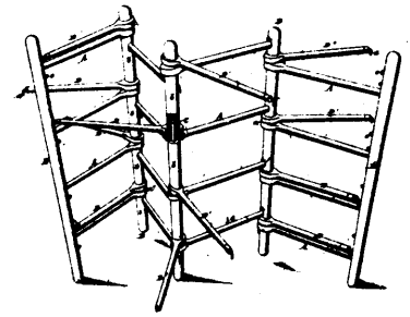
9644 Valley's Improvement on Clothes Driers.
