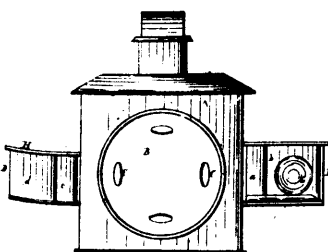
9654 Dressell & Voth's Improvements on Locomotive Head Lights
