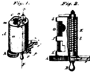
9641 Batchelder's Improvements on Repeating Matches
