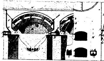
9649 Murphy's Improvements in Boiler Furnaces.
