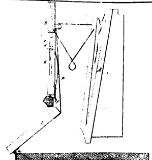
9656 White's Improvements on Organ Pedals.
