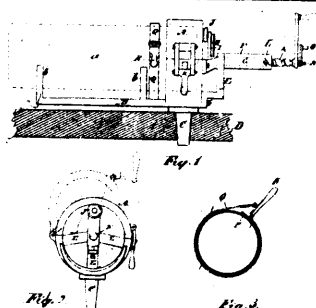
9652 Shirreff's Improvements on Screw-Thread Swaging Machines.
