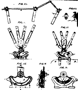
9642 No. 9642 Improvement on Reaping Tips
