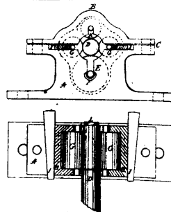
9655 McClory's Improvements on Shaft Bushes.
