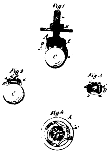
9651 Spencer's Improvements on Castors.
