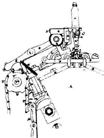
32195 Esty's Knitting Machine.
