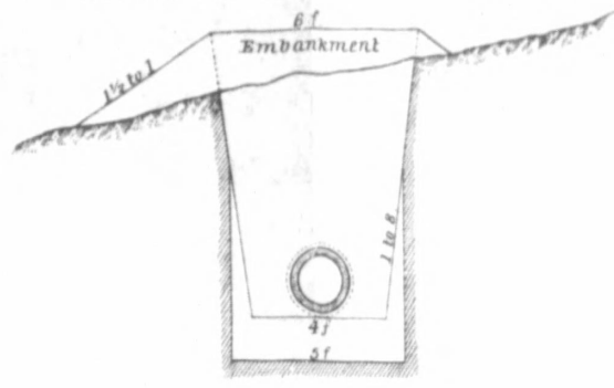
Section of Trench with Pipe in place
