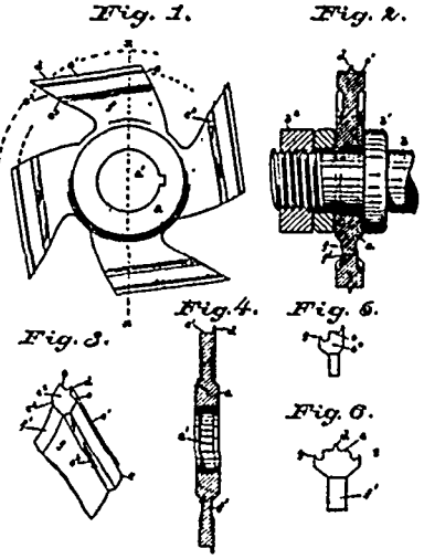
24478 Mahaffey's Cutter Head for Matching Machines.
