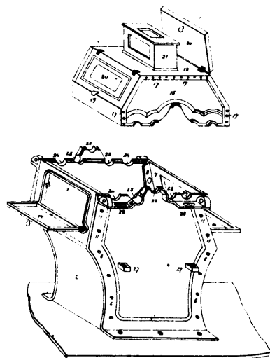
20247 Case's Casing for Roller Mill.
