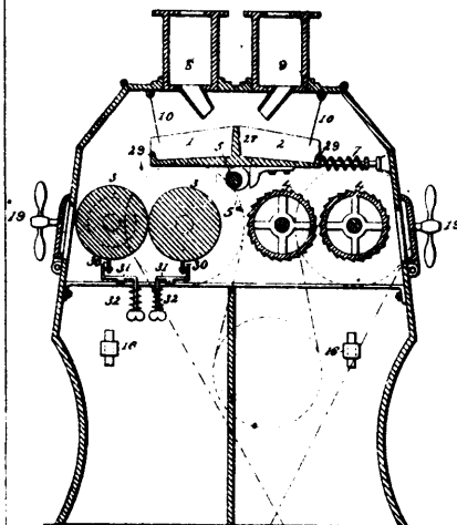
20249 Case's Feed Box for Roller Mill.
