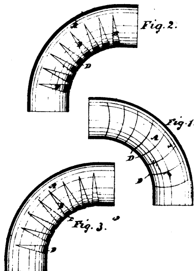
20242 Evans &amp; Bissett's Crimped Stove Pipe Elbow.
