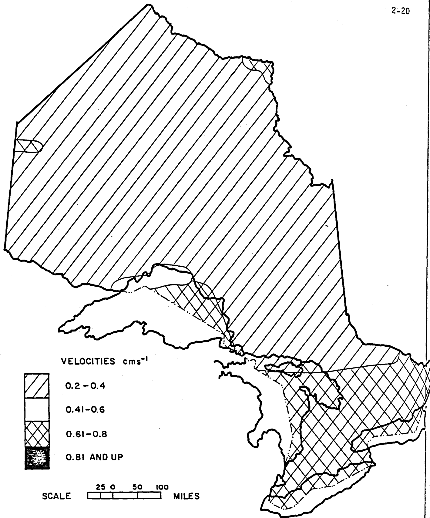
Figure 5: Deposition velocities of \text{SO}_2 for December-February.
