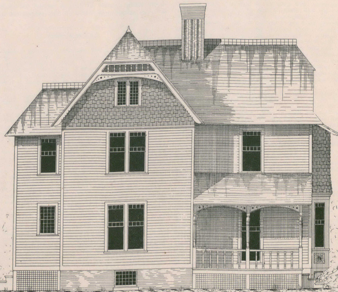
SIDE ELEVATION
