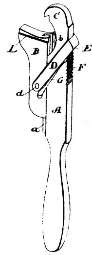
36039 Craig's Combined Nut and Pipe Wrench.
