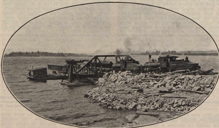
Canadian Northern Railway Rainy Lake Revision, Barges and Girders in use.
