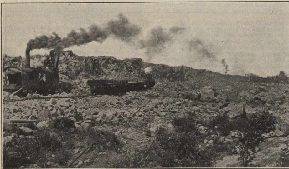
Canadian Northern Railway Rainy Lake Revision. Main Borrow Pit.
