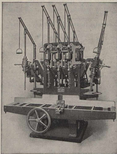
No. 327—Vertical Car Boring Machine with Universal Spindles
