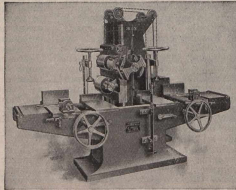
No. 525—Vertical Automatic Car Sill Tenoning Machine.
