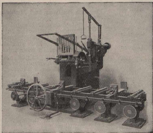
No. 512—Extra Range Automatic Car Gainer with Boring Attachment.
