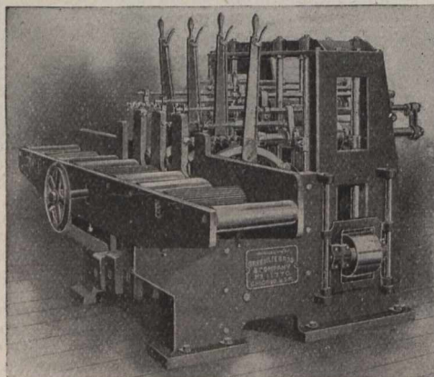
No. 306—Extra Range Horizontal Car Boring Machine.
