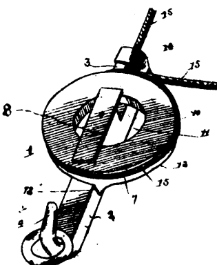
34526 Harvey's Draft Hook.
