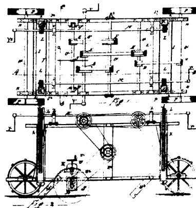
33971 Baxter's Implement for Cutting or Harvesting Ice.
