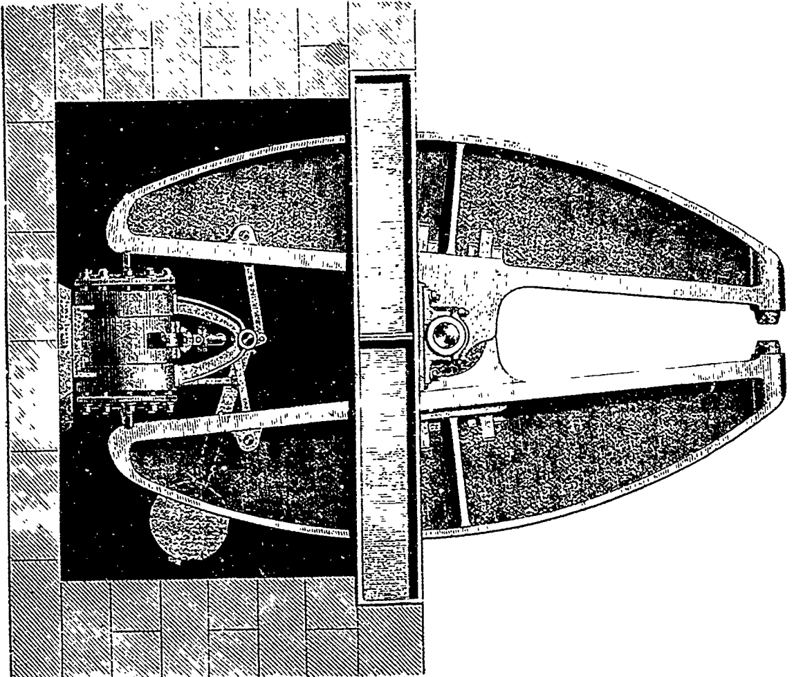
HYDRAULIC RIVETTING MACHINE.—(See page 380.)
