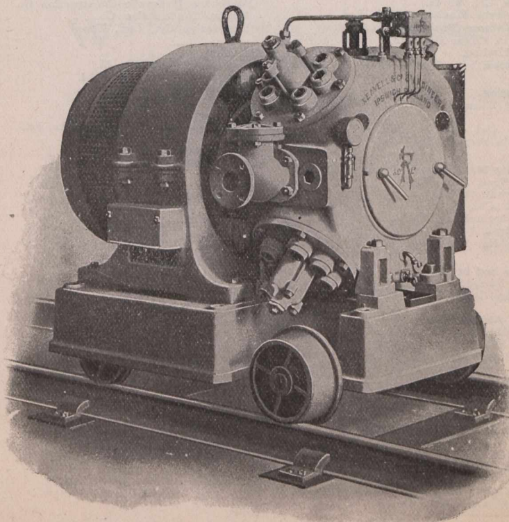
Direct Coupled Motor-Driven Compressor arranged on wheels for "In-Bye" working.
