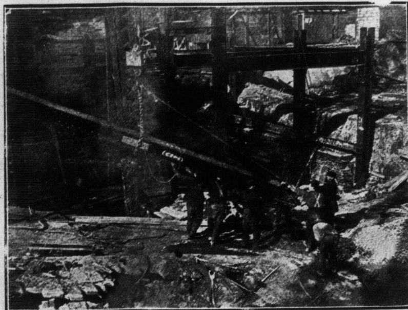
NEW TRUSTS AND GUARANTEE BUILDING. Workmen raising the steel girders and placing them in position. This handsome structure is being erected at the corner of Bay and Melinda-streets.
