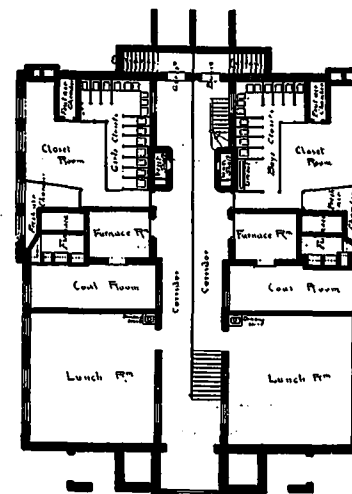
Basement Plan
