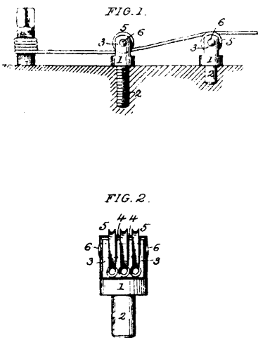
42025 Reed's Piano Agraffe.
