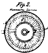
4130 Renshaw's Improvements on Superheaters
