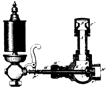
4132 Farnellee's Automatic Fire Extinguisher.
