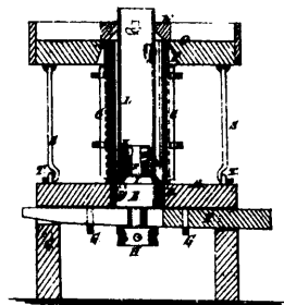
4139 Merwin's Improvements in Drain-pipe Moulding Machines.
