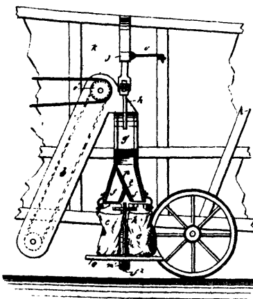
22148 Barber's Grain Sacking and Weighing Attachment for Thrashing Machines.
