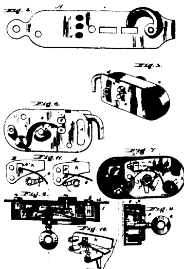
15869 Young's Improvements on Hasp Locks.
