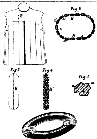
16213 Cogswell's Improvements on Life Preservers.
