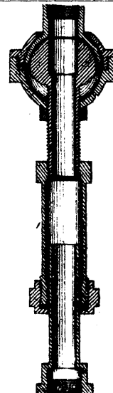
16222 Martin's Improvements on Pipe Couplings.
