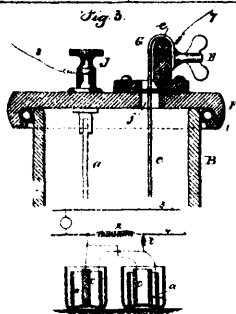
13208 Edison's Improvements on Velometers.
