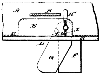
13223 Atwood's Improvements on Centre Boards for Boats.
