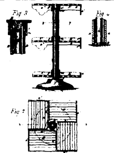
10954 Johnson's Improvements on Book Cases.
