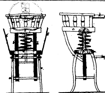
2797 Emmons & Keane's Improvements in Children's Chairs.
