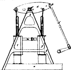
2795 Bartley's Improvements on Walking Beam Steam Engines.
