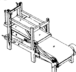
2801 Rouleau's Machine for Drying, Cleaning and Purifying Magnetic Sand.
