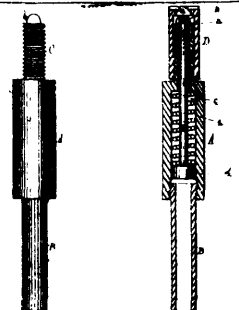
2615 Worden's Attachment to Steam Engine Lubricators.
