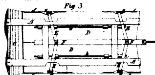
2611 Walker's Railway Snow Plow.
