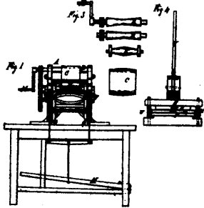
7379 Marengo's Process of Making Cigars and Cigarettes.
