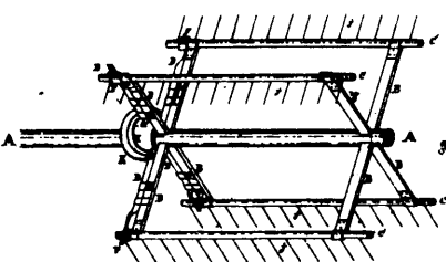
2225 Kumpf's Harvester Reel.
