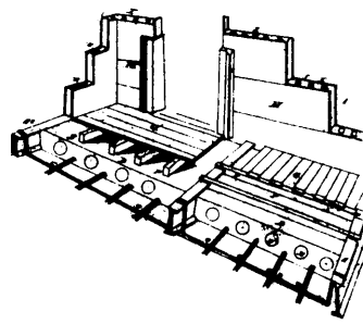
2230 Wright's Tubular Block Fire Proof Building Material.
