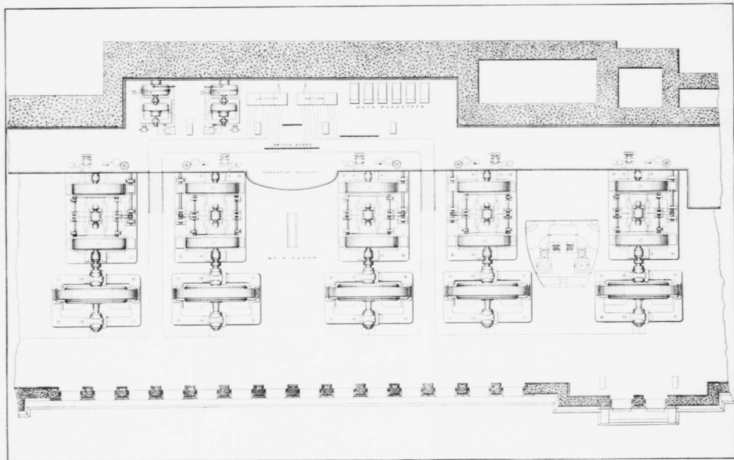
PLAN OF GENERATING STATION, UNITS 2 TO 6.
