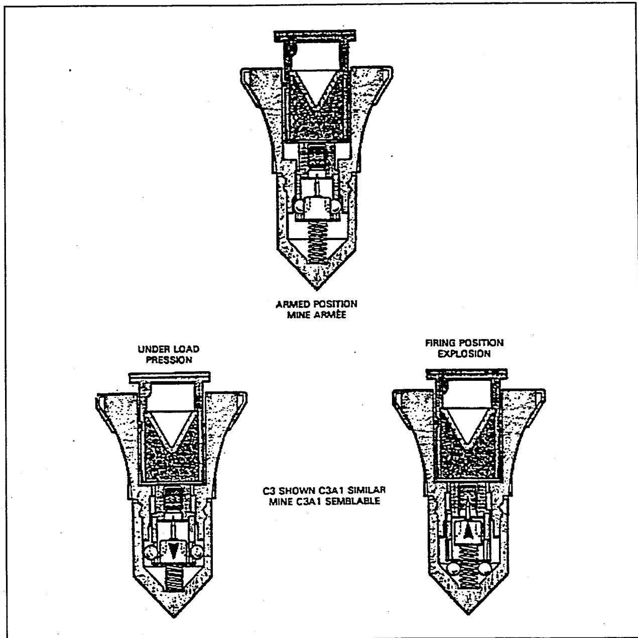
FIGURE 5 - FUNCTIONING OF ANTI-PERSONNEL MINE C3 AND C3A1
