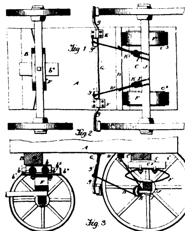
Criswell's Wagon Brake.
