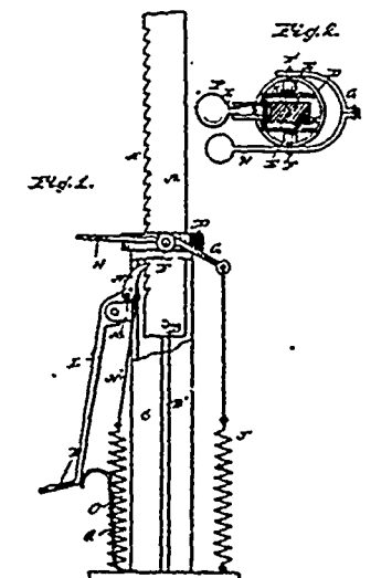
23951 Stuck's Lowering Mechanism for Dentists' Chairs.
