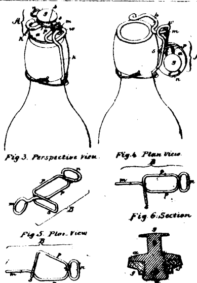
21043 Lloyd's Bottle Stopper.
