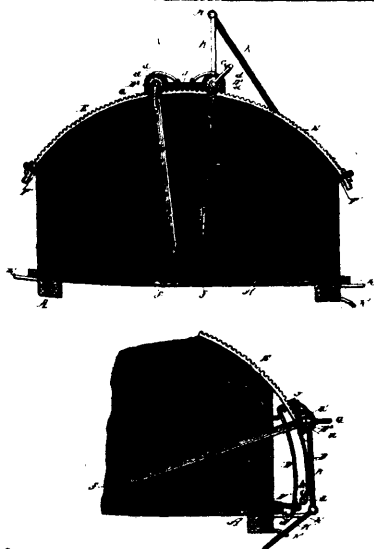
21035 Wyman's Railway Car Cover.
