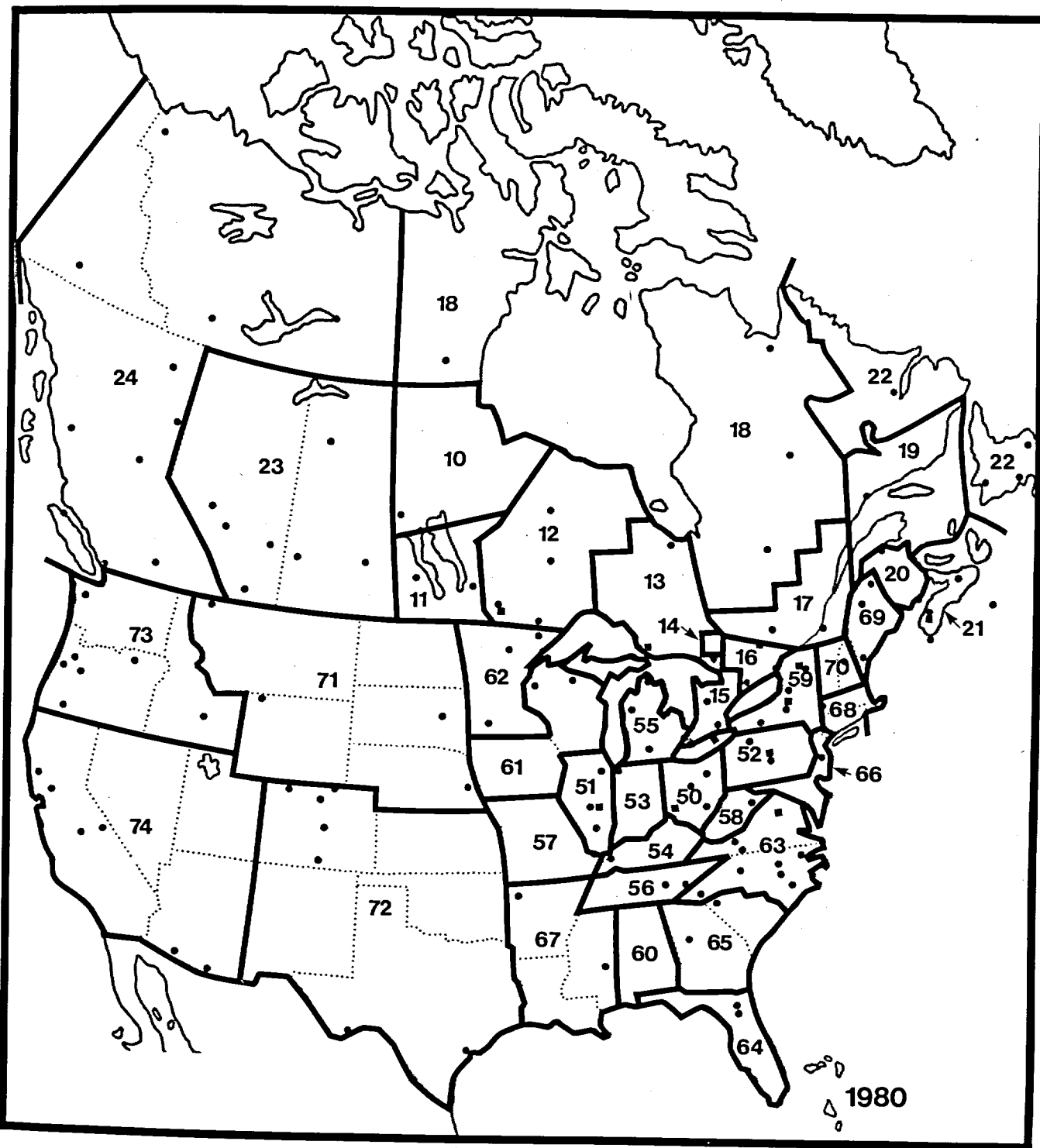
North American source regions used for the transfer matrices
