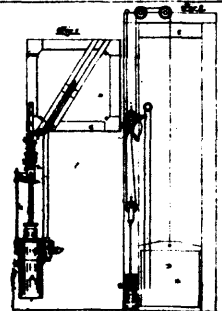
5025 Fensom's Hydraulic Elevator.
