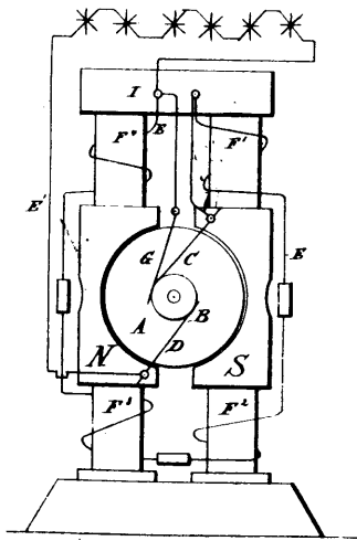
30937 Waterhouse's Dynamo Electrical Machine.
