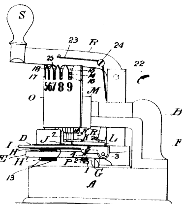
30941 Smith &amp; Williamson's Check Punch.
