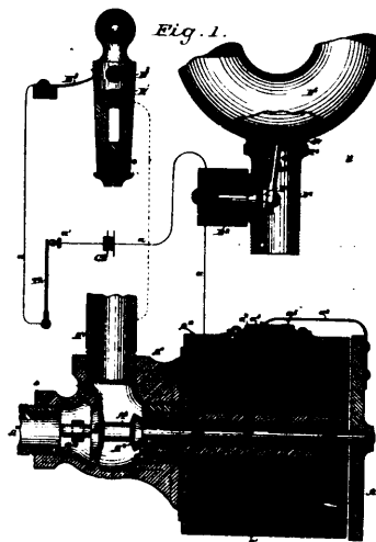
30938 Newman's Electro Thermostatic Anti-Freezing Apparatus.
