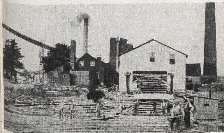
Log Hoist and Slasher House at the receiving end of a Pulp Wood Storage System.
