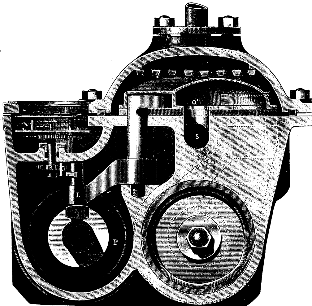
FIG. 1.—VERTICAL SECTION.
