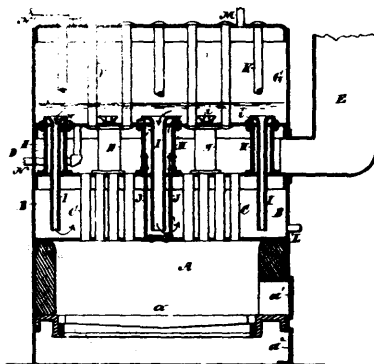
36828 Tonn's Steam Generator.
