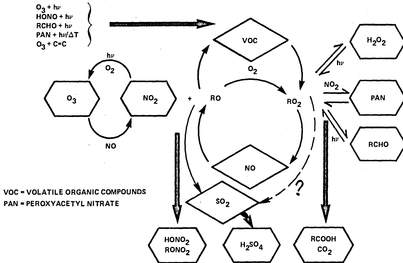
FIGURE 4.2 Schematic of the polluted atmospheric gas-phase photooxidation cycle
