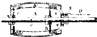
12078 Wright's Improvements on Barrel Forming Machines.
