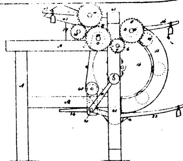
12079 Waddell's Improvements on Barrel Machinery.
