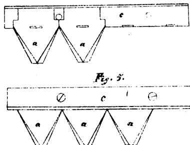
12074 Montrose's Improvements on Cutter Bars for Harvester.
