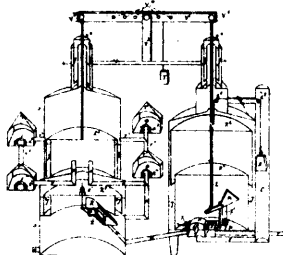
8170 Hicks' Improvements on Gas Governors.
