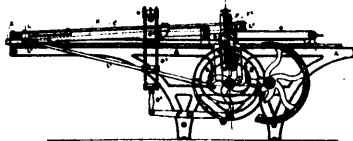
8173 Robertson's Improvements on Lozenge Machines.
