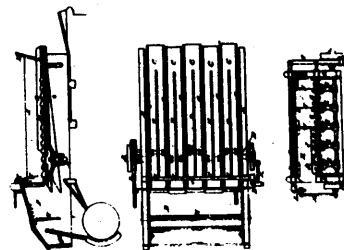
3327 Wilders' Improvements on Threshing Machines.
