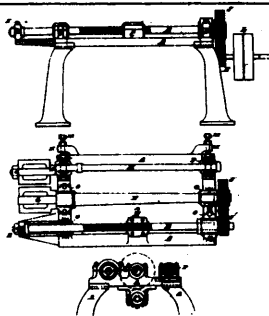
3326 Mackenzie's Machine for Making Spiral Springs.
