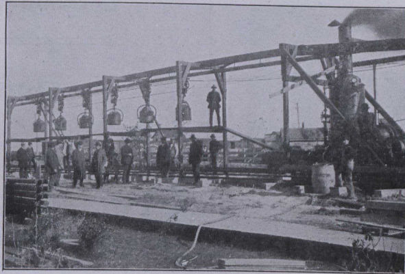
CARSON TRENCH MACHINE At Winnipeg, Man.
