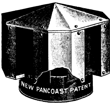
PANCOAST VENTILATOR.
