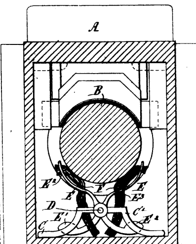
27870 Nichol's Axle Lubricator.
