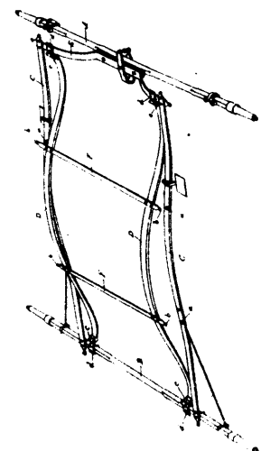
27872 Armstrong's Side Bar Side Spring Buggy Gear.
