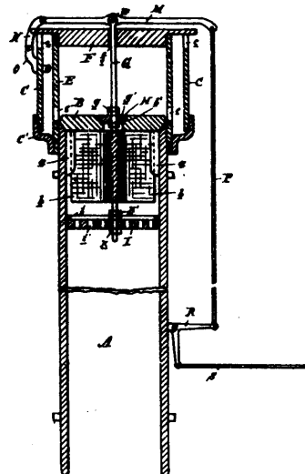
27871 Lozon's Throttle Valve for Locomotives.
