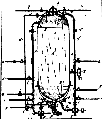
27864 Tompkins' Apparatus for Making Paper Stock.
