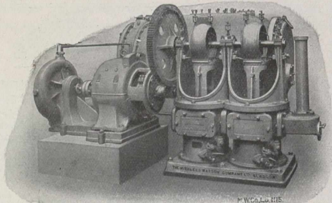
Surface Condenser with 2-throw Edwards Air Pump and Centrifugal Circulating Pump
