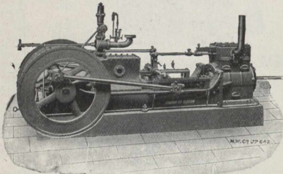
Steam Driven Dry Air Pump
