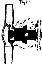
10331 Porteous's Improvements on Stop and Waste Cocks.
