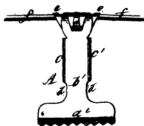
10336 Greig's Improvements on Clasps.
