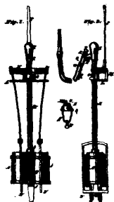
10333 Howe's Improvements in Submerged Pumps.
