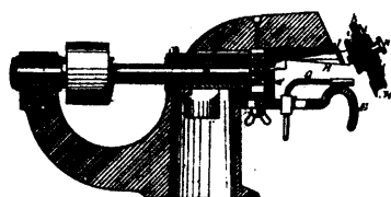
7768 Fullerton's Machine for Setting the Edges of Boots and Shoes.
