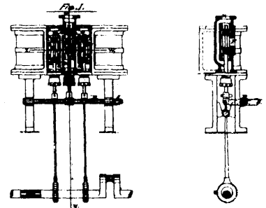
2096 Glen's Reversing Valve and Steam Chest.
