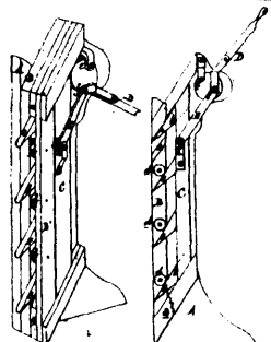
2102 Fordon's Dogs for Circular Saw Mills.
