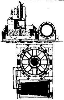
2100 Howland &amp; Taft's Machine for reducing Wood to Pulp.
