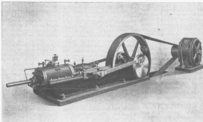
One of our 12 \frac{1}{4} x 18 "Ingersoll" Air Compressors driven by one of our 50 h. p. Induction Motors and supplying power for a western quarry. Catalogue No. 75 describes and illustrates the different classes of our Air Compressors and the uses to which they are best adapted.
